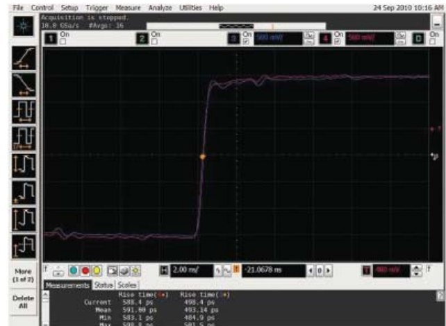
Time domain step response of N2796A (with Agilent MS09404A)
