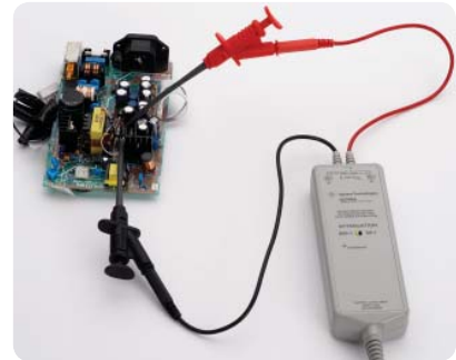
N2790A measuring a power supply signal
